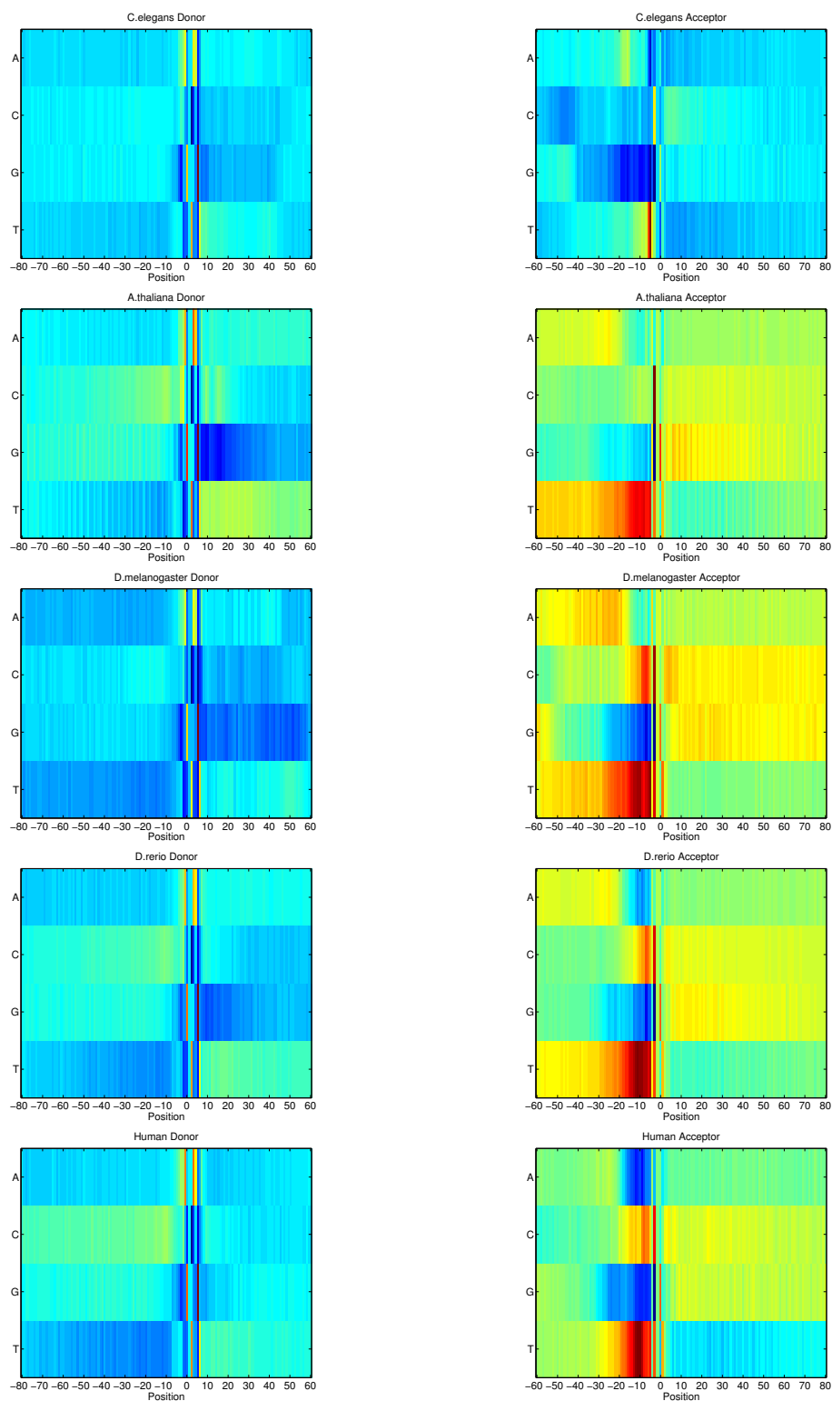
Figure 1: POIMs (Positional Oligomer Importance Matrices) for single nucleotides comparatively for worm, cress, fly, fish, and human. Position 1 denotes the splice site and the start of the consensus dimer.
