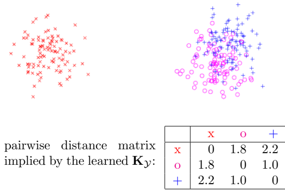
Figure 4: Toy experiment for learning k_Y .
